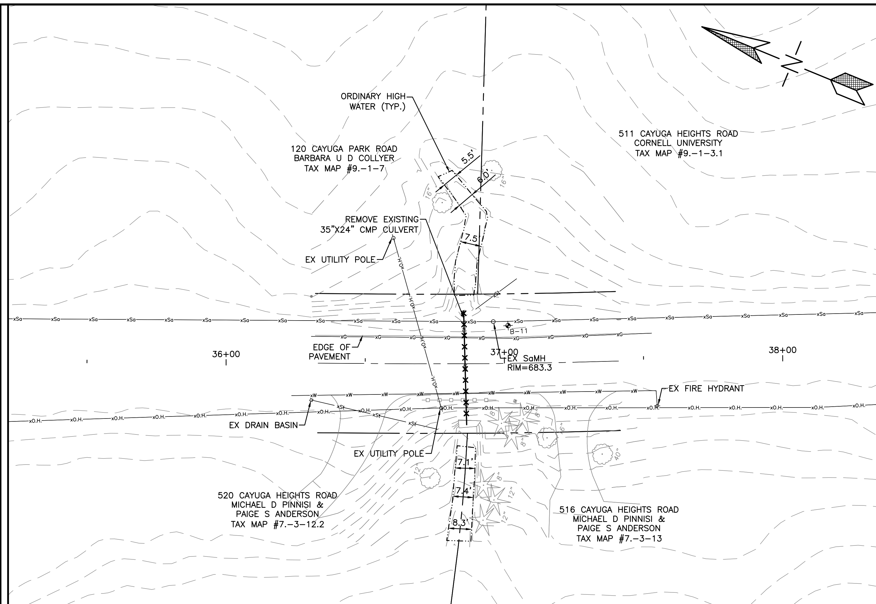
1 EXISTING CONDITION - CULVERT 9 SCALE 1"=20'
