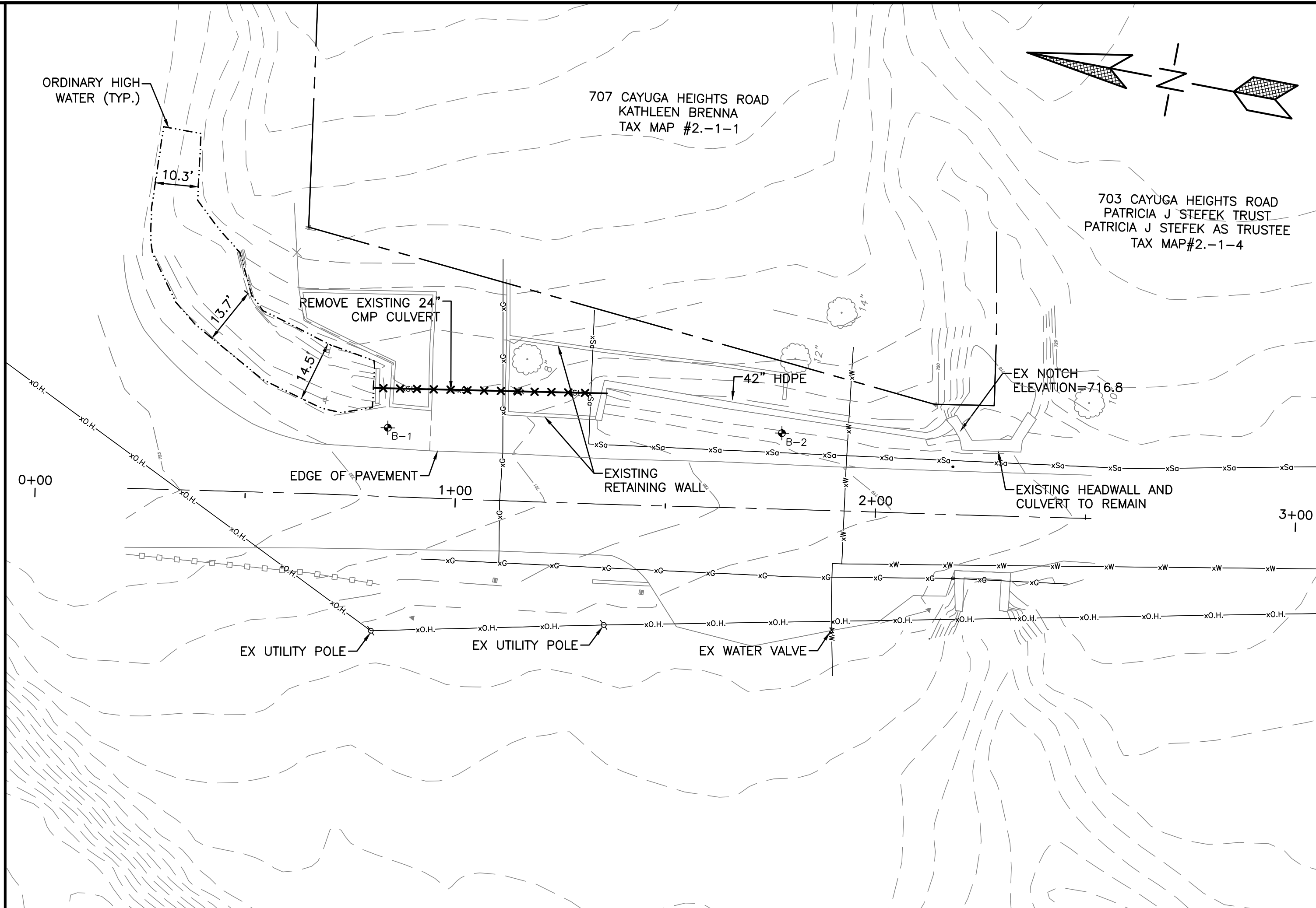
1 EXISTING CONDITION - CULVERT 1 SCALE 1"=20'
