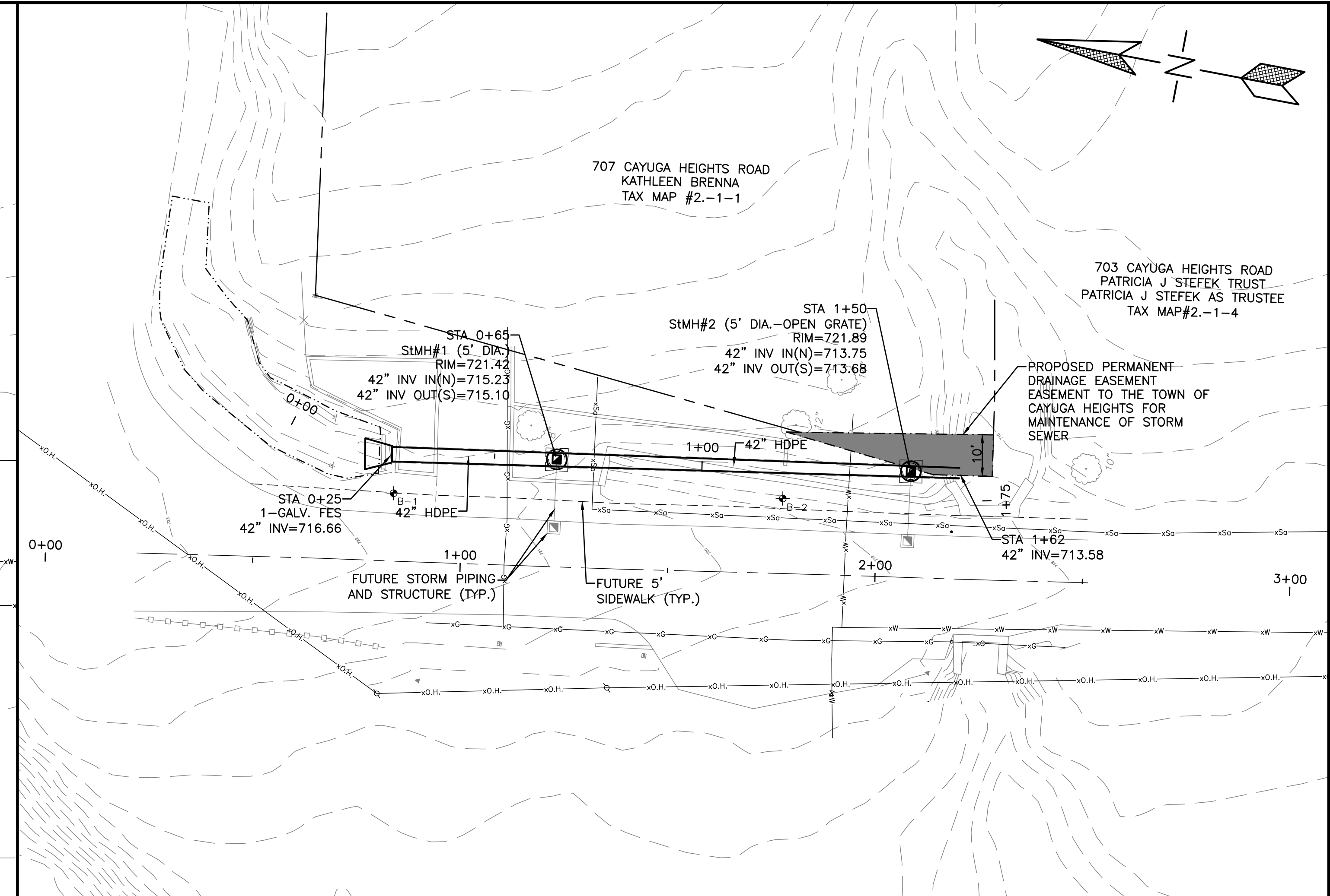
2 LAYOUT PLAN - CULVERT 1 SCALE 1"=20'
