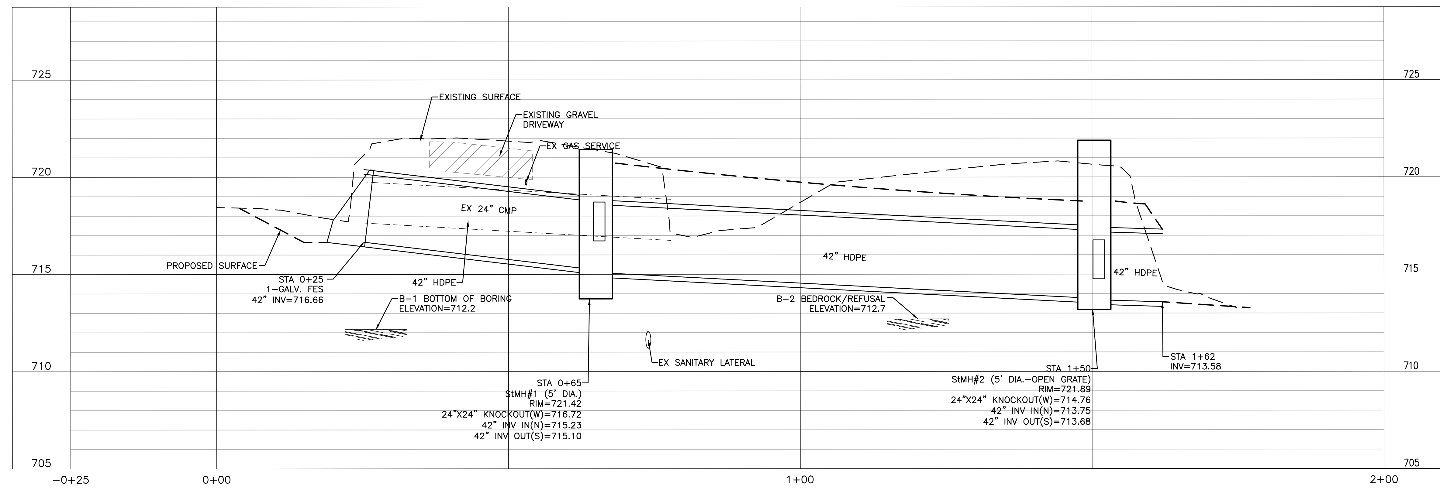
3 PROFILE - CULVERT 1 SCALE H: 1"=10' V: 1"=3'
