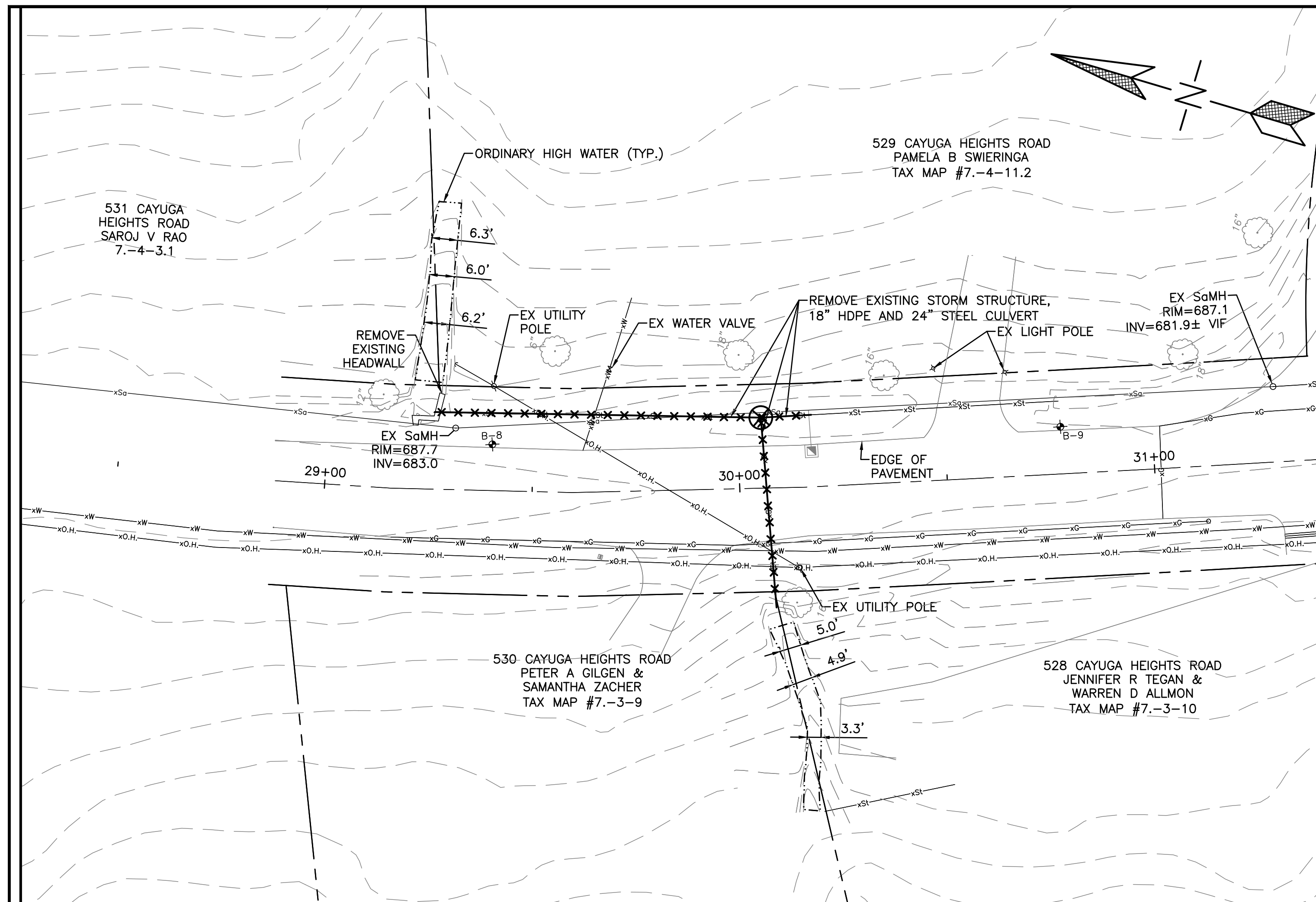
1 EXISTING CONDITION - CULVERT 7 SCALE 1"=20'
