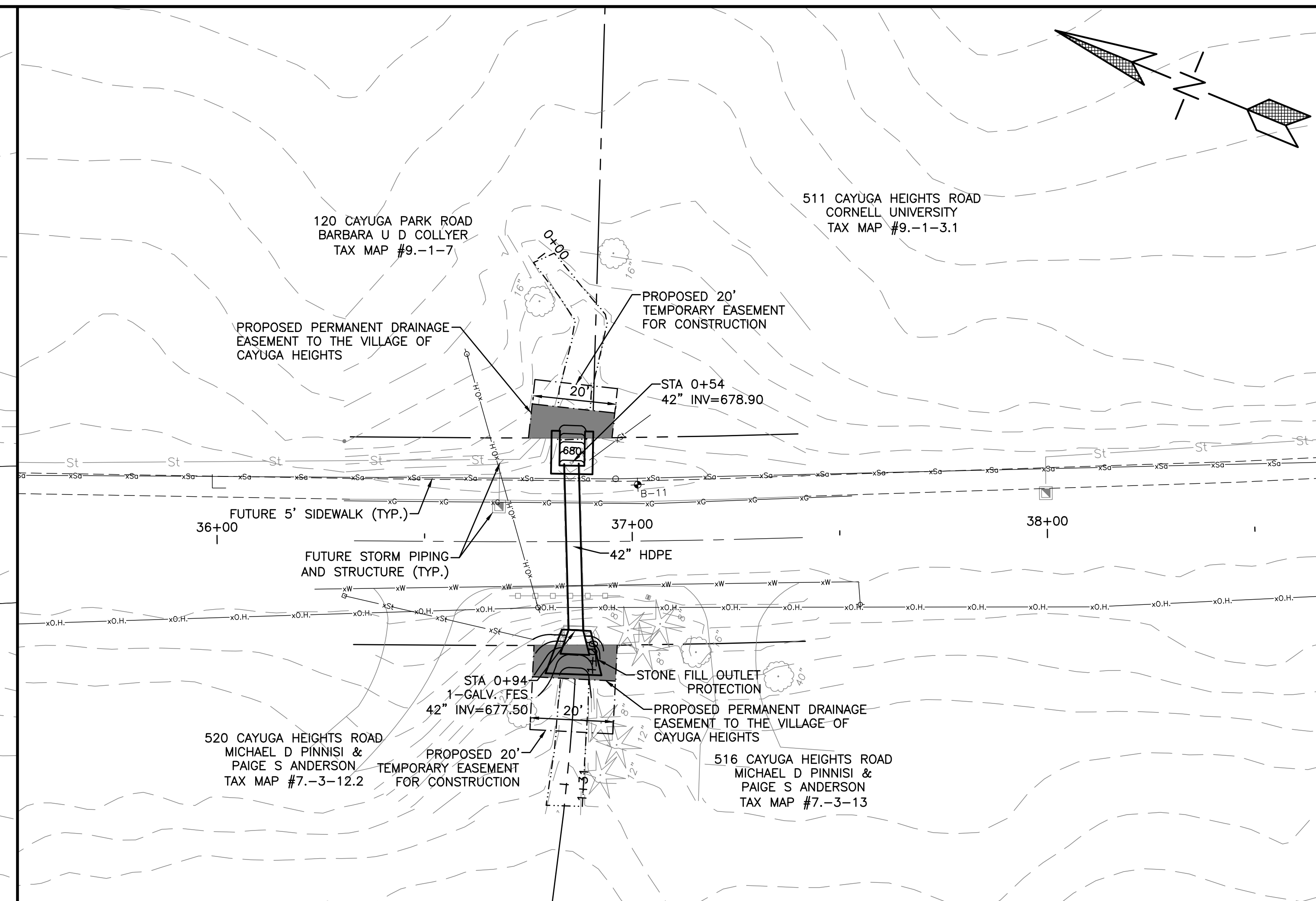
2 LAYOUT PLAN - CULVERT 9 SCALE 1"=20'
