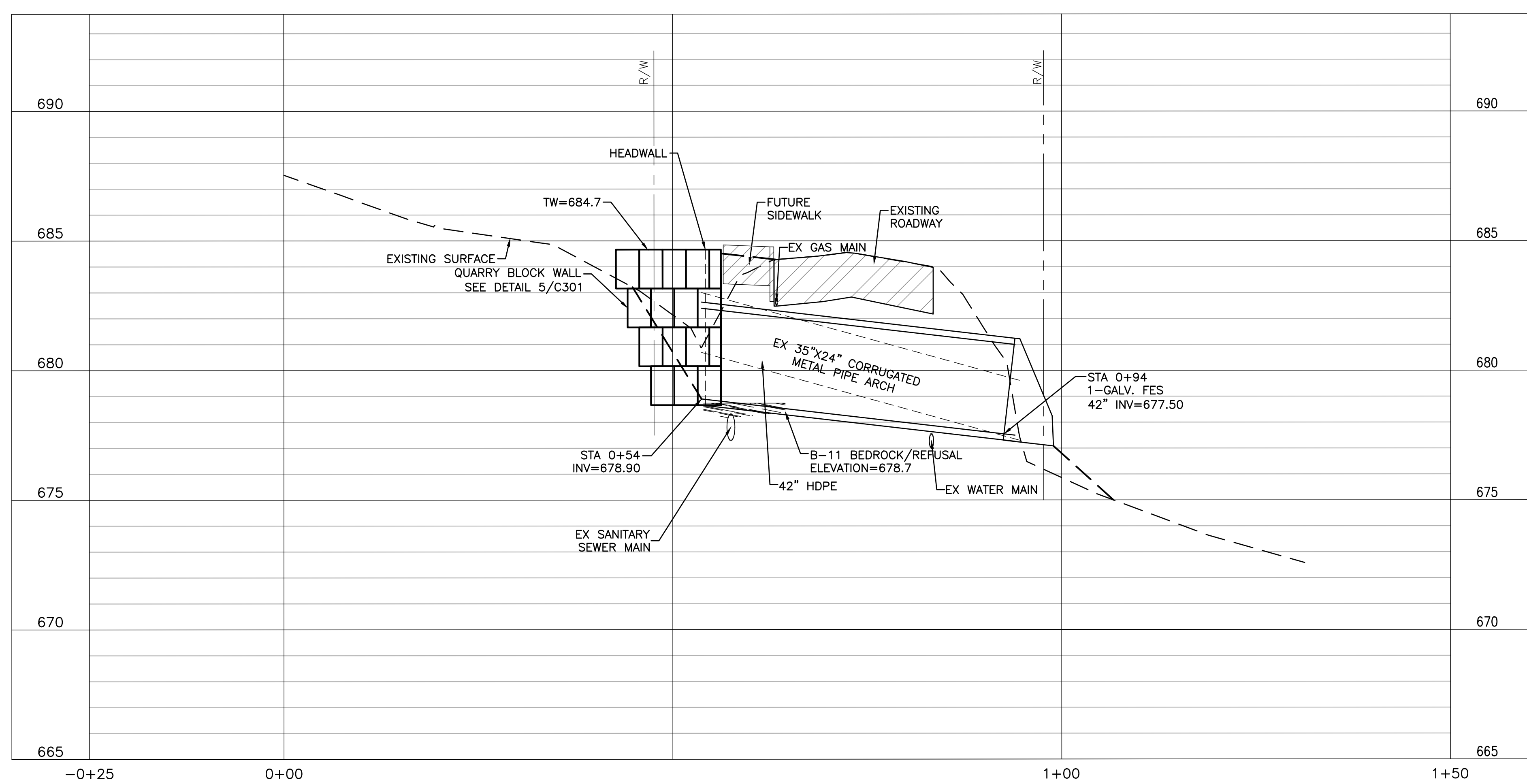
1 EXISTING CONDITION - CULVERT 9 SCALE 1"=20'
