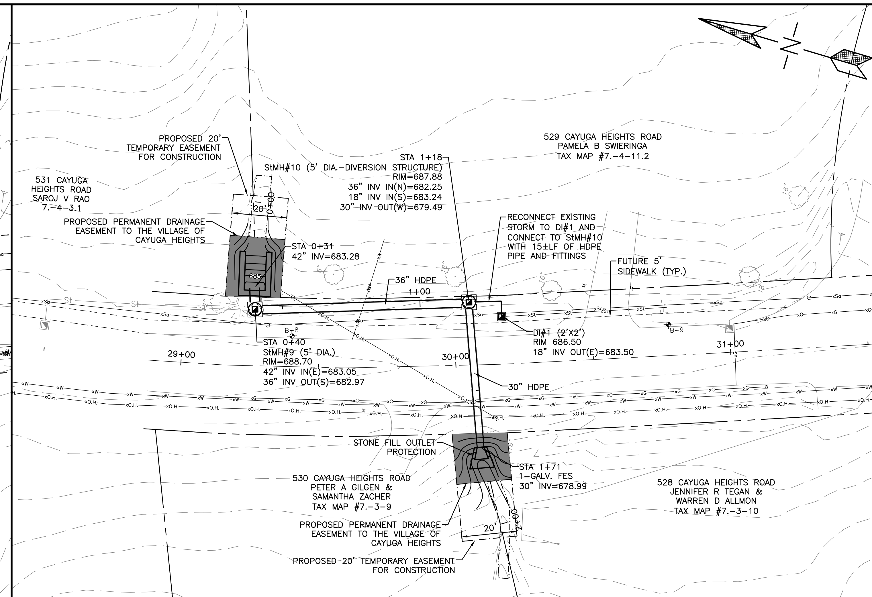
2 LAYOUT PLAN - CULVERT 7 SCALE 1"=20'
